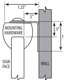
Channel Bracket
